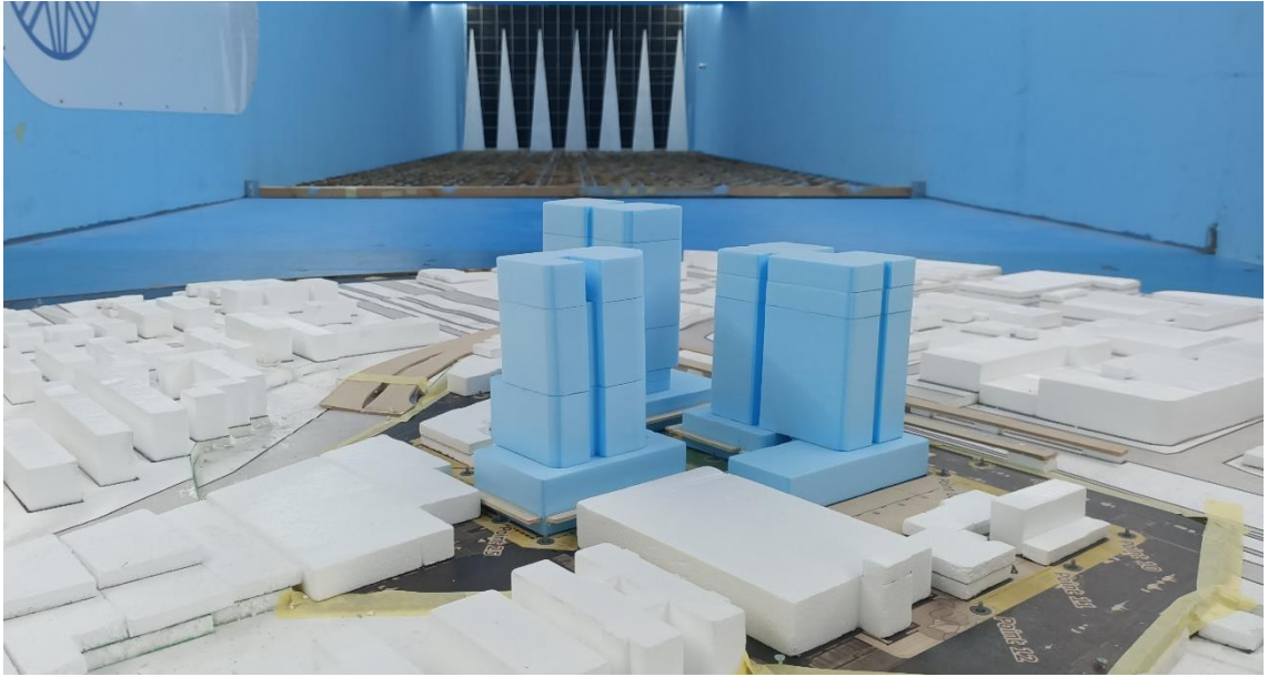
Figure 1f: Photograph of the Wind Tunnel Model (close-up view from the north)
