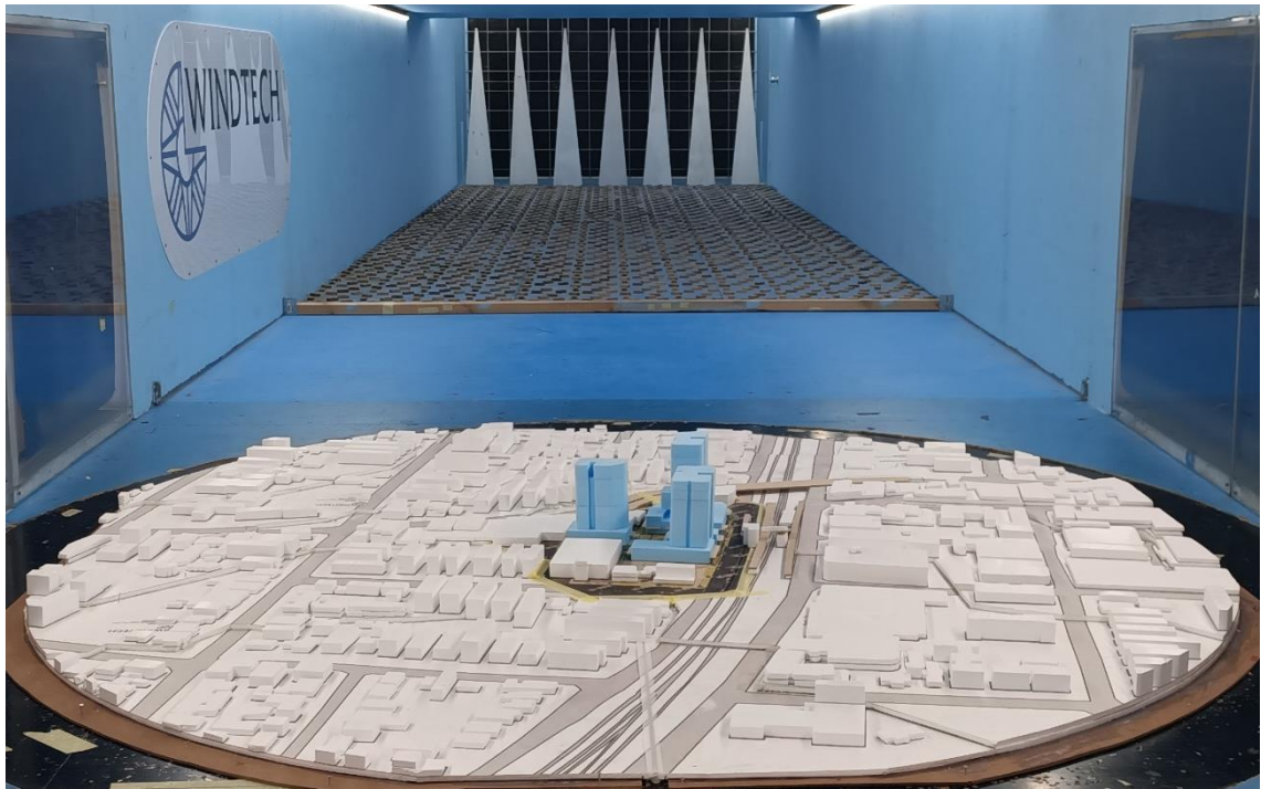
Figure 1d: Photograph of the Wind Tunnel Model (view from the north)
