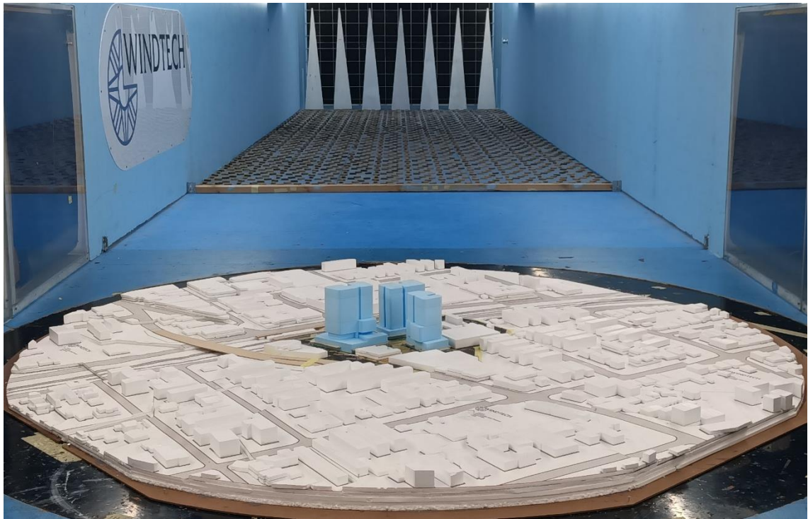
Figure 1b: Photograph of the Wind Tunnel Model (view from the south-east)
