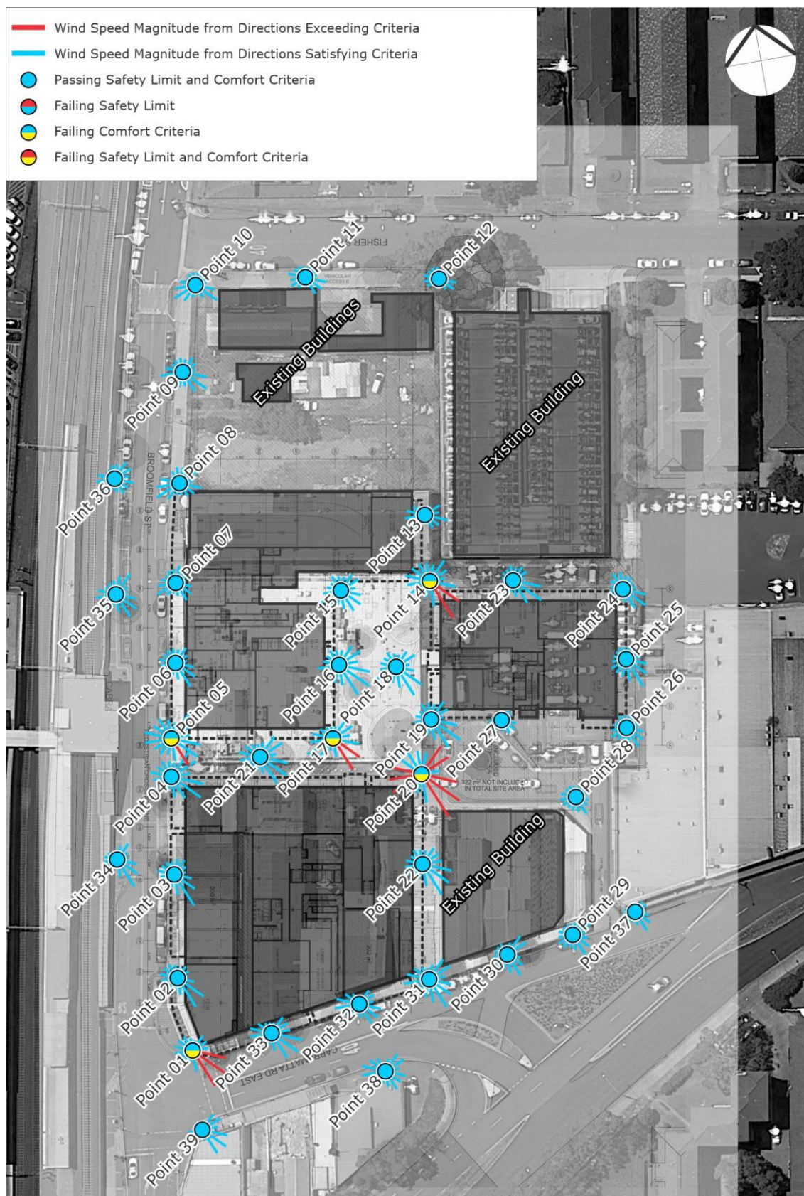
Figure 6: Wind Tunnel Results – Ground Level Plan (results shown without treatments applied)
