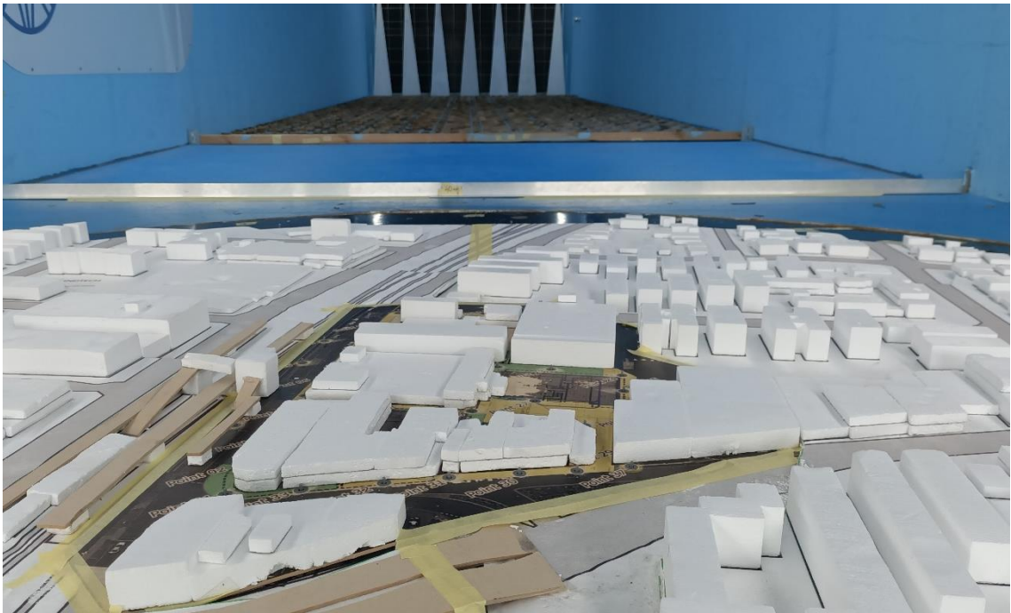
Figure 1i: Photograph of the Wind Tunnel Model (close-up view from the south (existing case))
