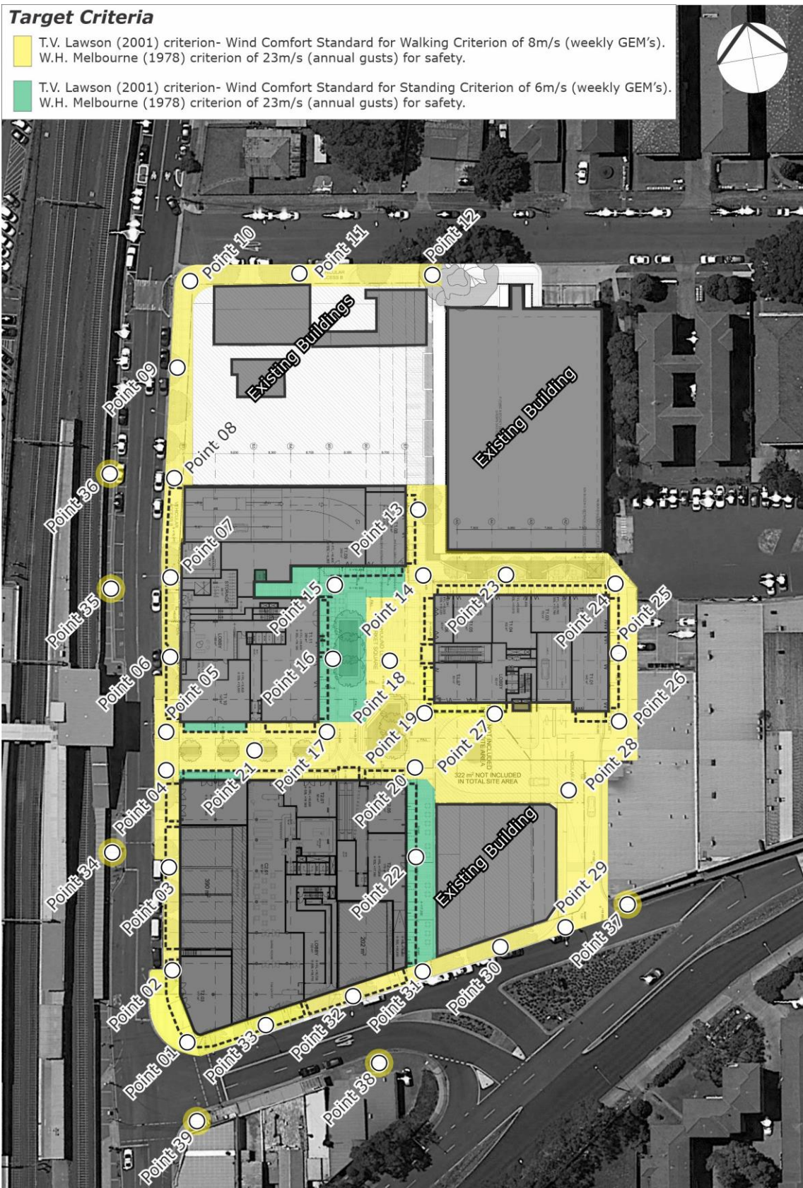
Figure 5: Study Point Locations and Target Wind Speed Criteria – Ground Level Plan
