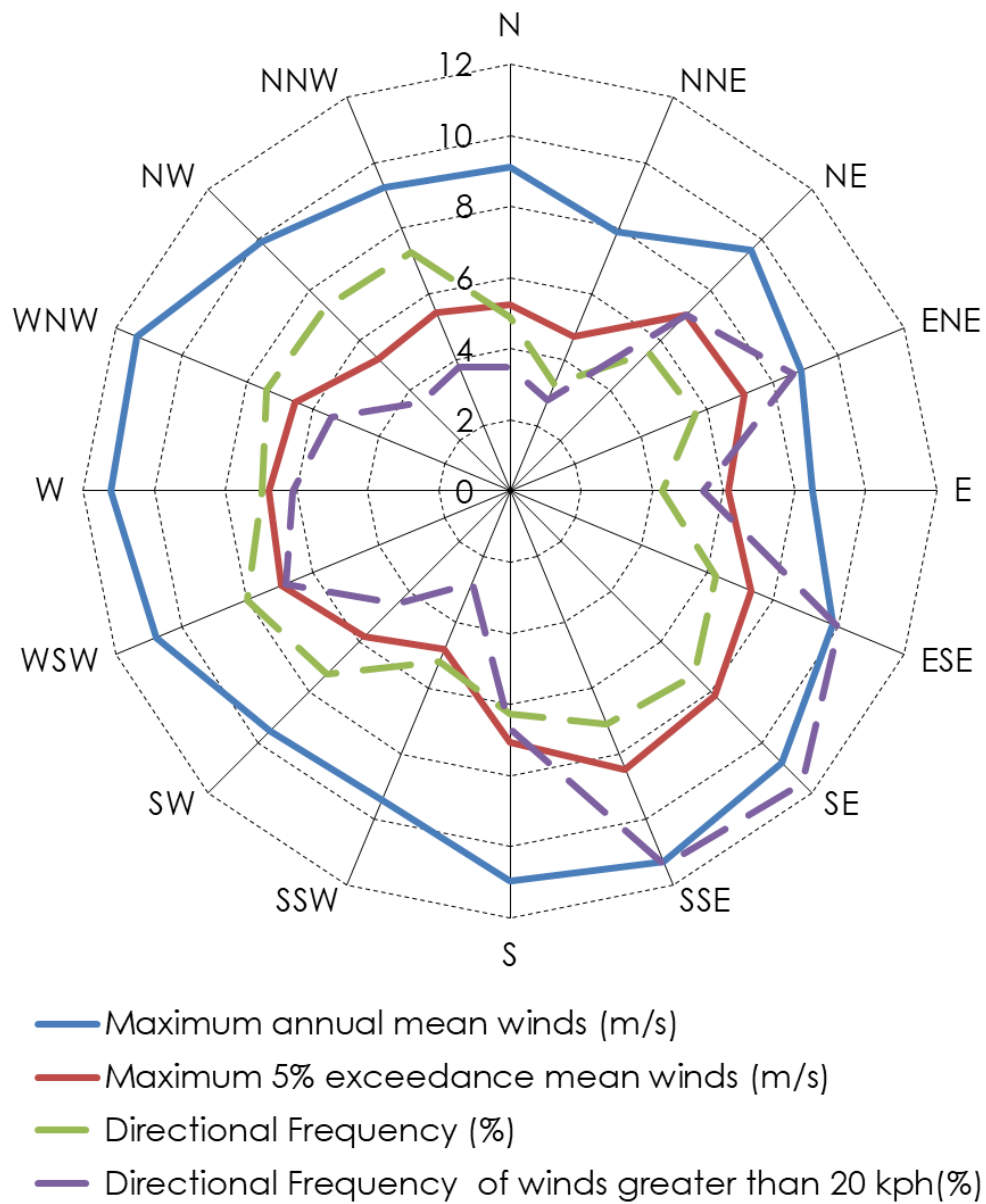
Figure 4: Annual and 5% Exceedance Hourly Mean Wind Speeds, and Frequencies of Occurrence, for the Bankstown Region (at 10m height in standard open terrain)
