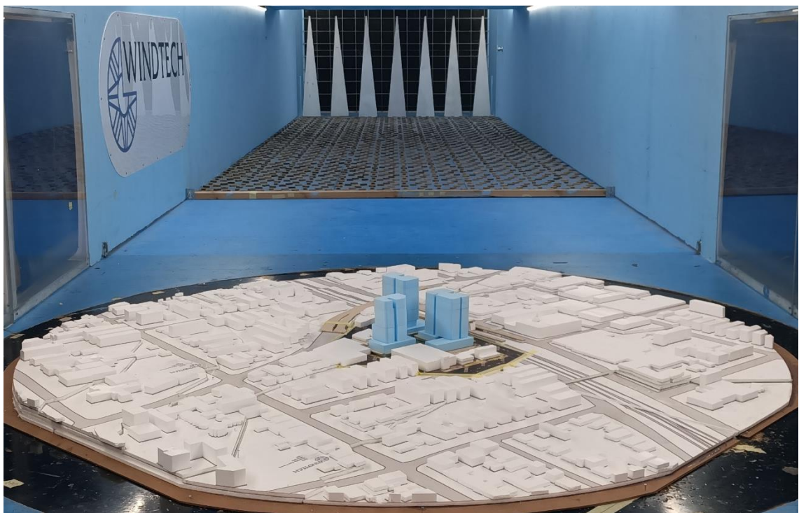
Figure 1c: Photograph of the Wind Tunnel Model (view from the north-east)
