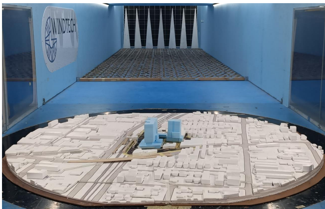
Figure 1a: Photograph of the Wind Tunnel Model (view from the south)
