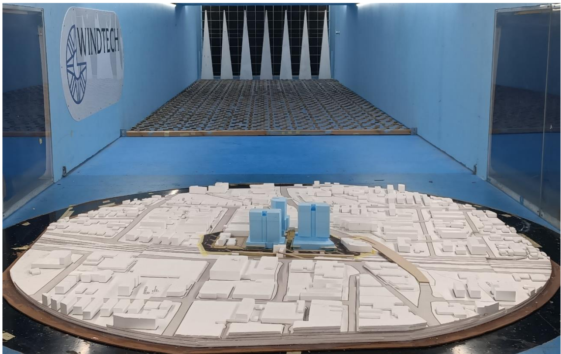
Figure 1e: Photograph of the Wind Tunnel Model (view from the west)
