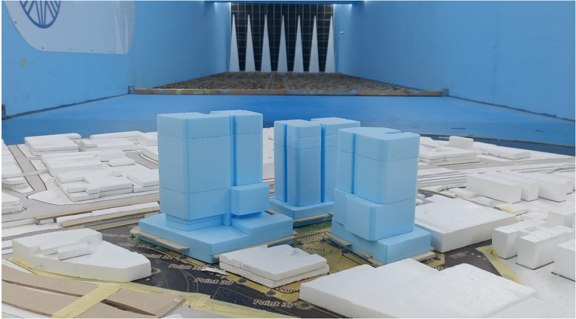
Figure 1h: Photograph of the Wind Tunnel Model (close-up view from the south-east)
